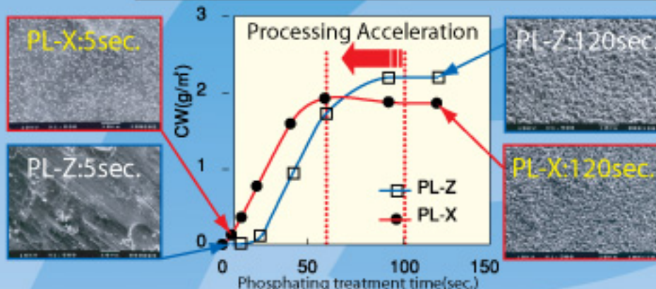
Treatment time and Coating Morphology Relation between phosphating treatment time and coating morphology
