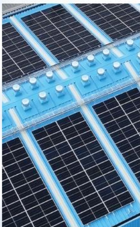
Solar cell
